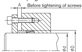
Assembly 2
