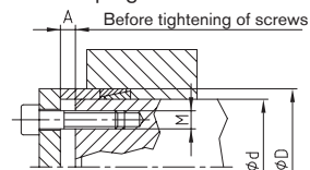
Clamping on shaft side
