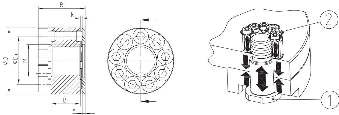
Clamping nut
