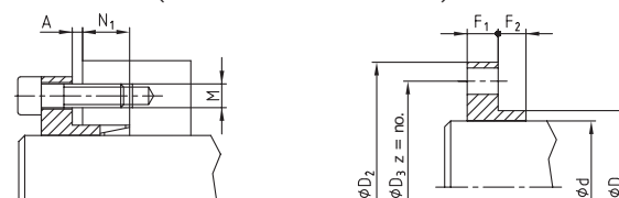
Recommended pressure flanges* (dimensions see table below)
